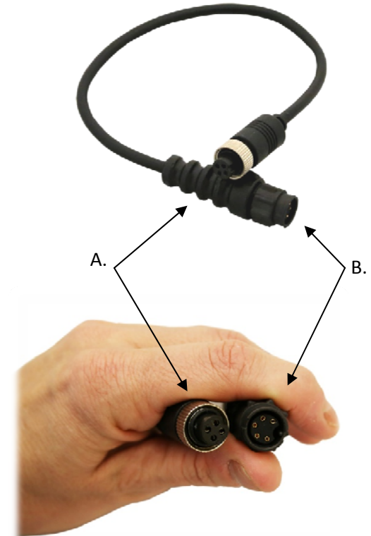
A. 4-Pin Female OverView Connector B. 5-Pin Female Switchcraft Connector
